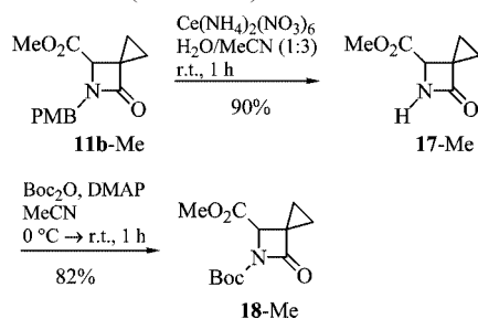
Scheme 3. Modification of the \beta -lactam 11b-Me to yield the reactive building block 18-Me .
