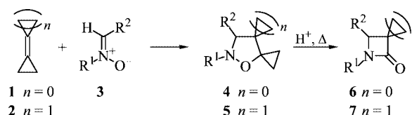
Scheme 1. Fragmentations of the cycloadducts 4 , 5 of nitrones 3 to methylenecyclopropane ( 1 ) and bicyclopropylidene ( 2 ) under acidic conditions.
