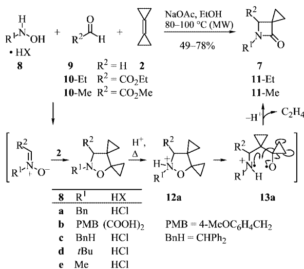
Scheme 2. One-pot three-component reaction under microwave heating for the direct conversion of alkylhydroxylamine hydrochlorides 8 , aldehydes 9–10 and bicyclopropylidene ( 2 ) to 3-spirocyclopropanated 2-azetidinones 7 and 11 . For details see Table 1.
